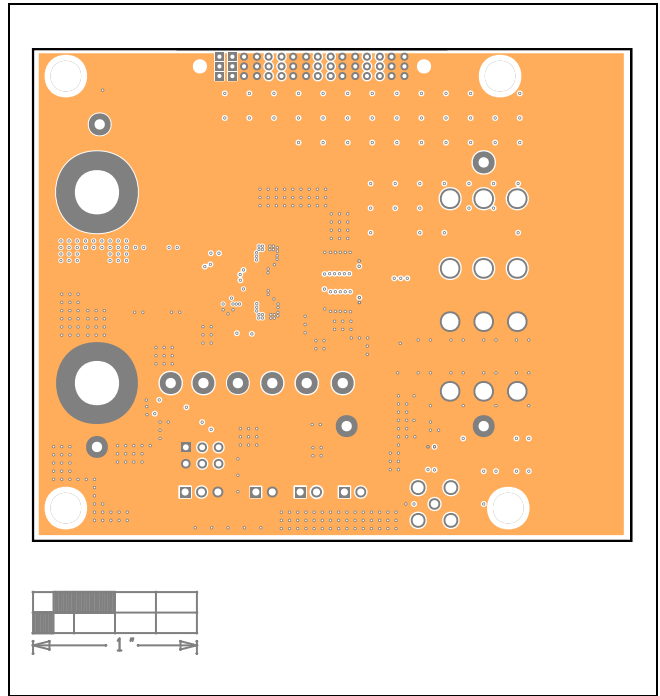
MAX20807 EV Kit PCB Layout—Layer 5
