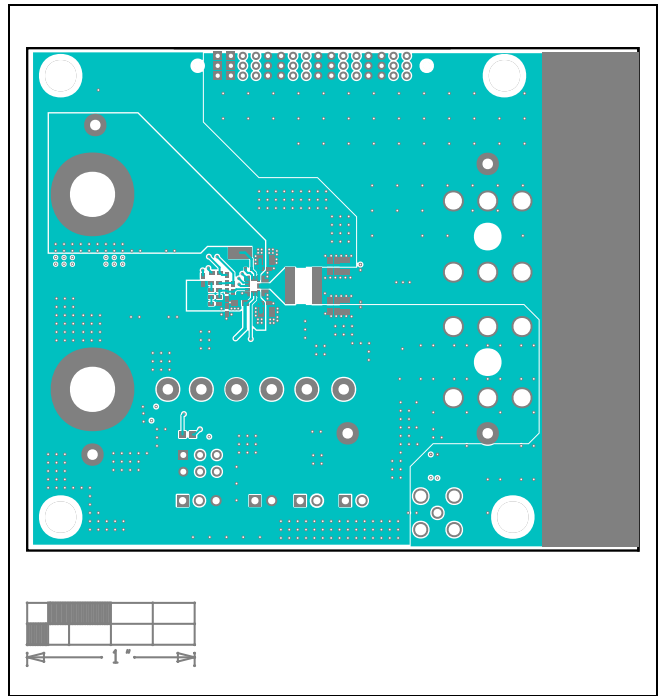
MAX20807 EV Kit PCB Layout—Top
