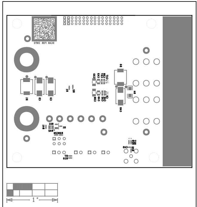
MAX20807 EV Kit Component Placement Guide—Bottom Silkscreen
