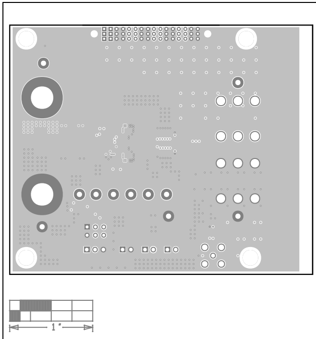
MAX20807 EV Kit PCB Layout—Layer 2
