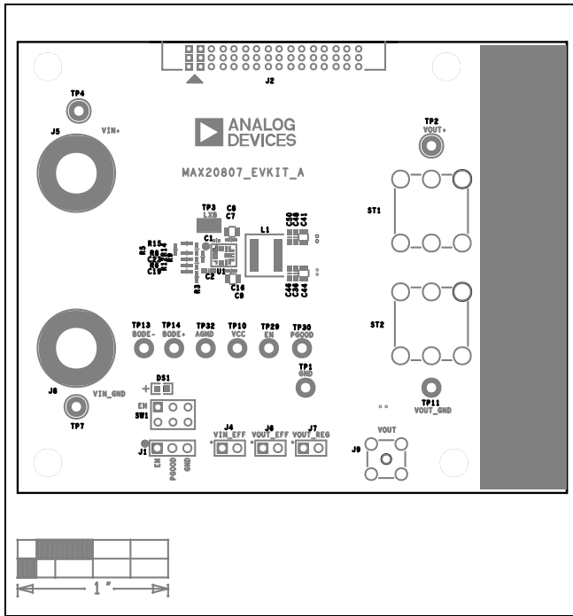
MAX20807 EV Kit Component Placement Guide—Top Silkscreen
