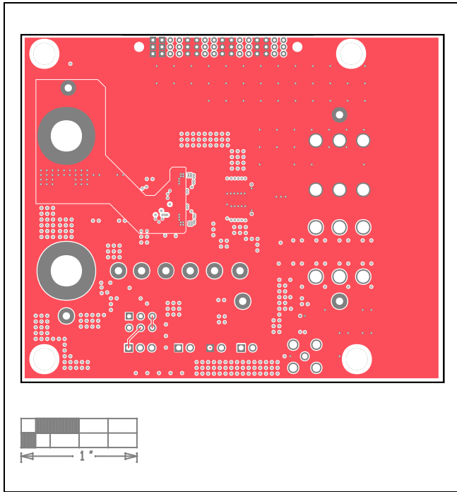
MAX20807 EV Kit PCB Layout—Layer 4
