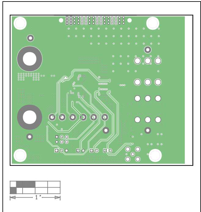
MAX20807 EV Kit PCB Layout—Layer 3
