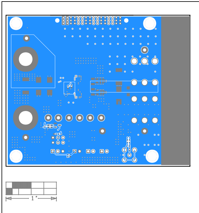
MAX20807 EV Kit PCB Layout—Bottom
