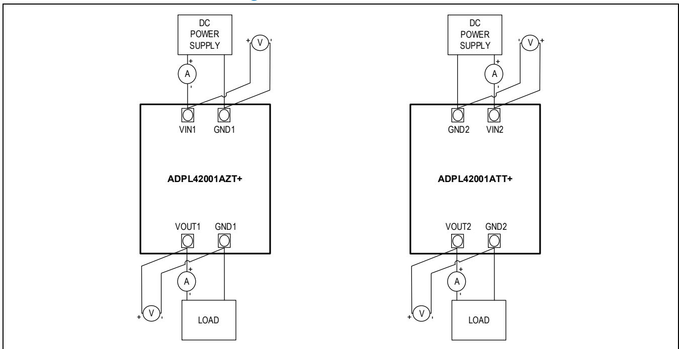
Figure 1. ADPL42001 EV Kit Connections
