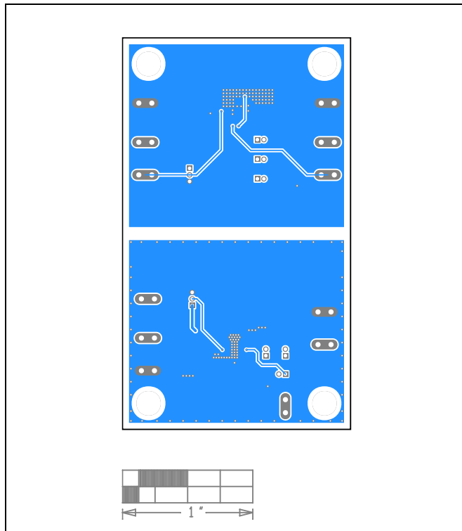
ADPL42001EVKIT—Layer 1
