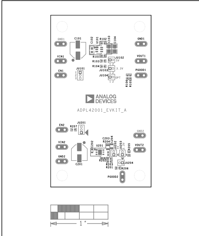
ADPL42001EVKIT—Top Silkscreen
