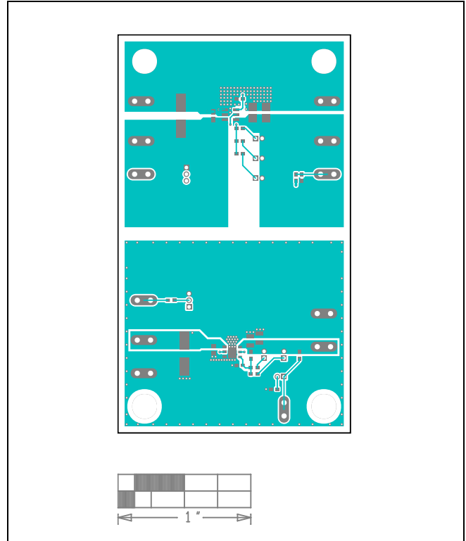
ADPL42001EVKIT—Layer 1
