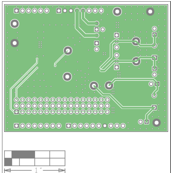
MAX33048E Shield EV Kit PCB Layout—Third Layer
