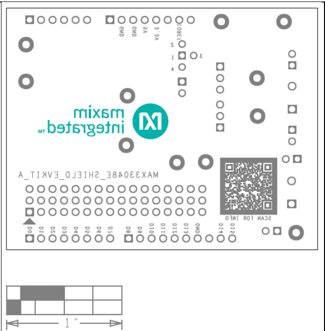
MAX33048E Shield EV Kit PCB Layout—Bottom Silkscreen
