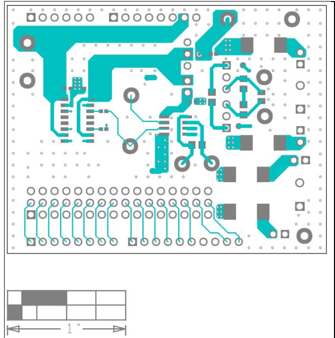
MAX33048E Shield EV Kit PCB Layout—Top Layer
