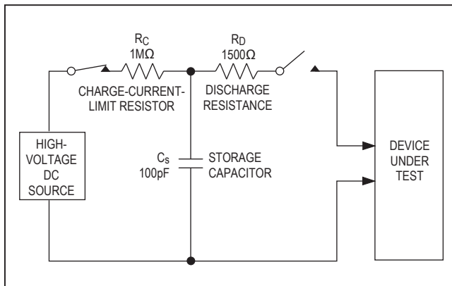
Figure 10a. Human Body ESD Test Model
