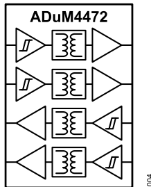
Figure 4. ADuM4472
