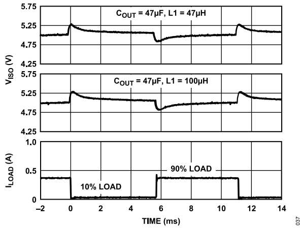
Figure 37. Typical V_{ISO} Load Transient Response 5 V Input to 5 V Output at 10% to 90% of 400 mA Load at 500 kHz f_{SW} with 0.1 \mu F Feedback Capacitor
