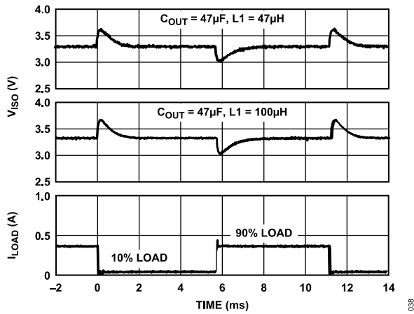
Figure 38. Typical V_{ISO} Load Transient Response 5 V Input to 3.3 V Output at 10% to 90% of 400 mA Load at 500 kHz f_{SW}
