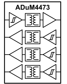
Figure 5. ADuM4473
