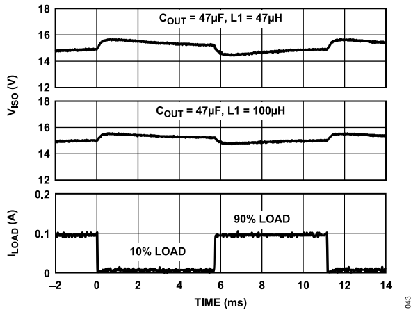
Figure 43. Typical V_{ISO} Load Transient Response 5 V Input to 15 V Output at 10% to 90% of 100 mA Load at 500 kHz f_{SW} with 0.1 \mu F Feedback Capacitor
