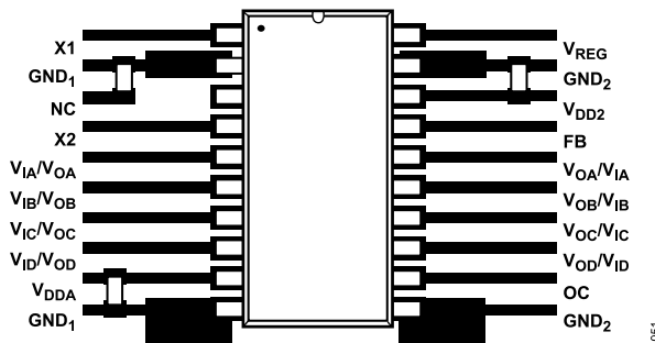
Figure 51. Recommended PCB Layout
