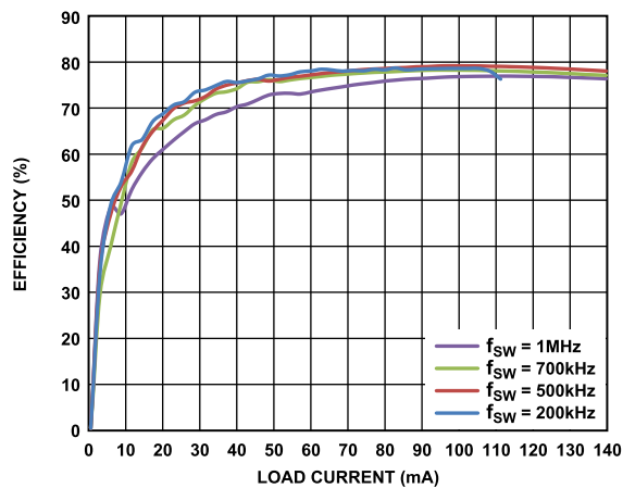
Figure 21. 5 V Input to 15 V Output Efficiency at Various Switching Frequencies with 1:3 Halo Transformer (TGSAD-290V8LF)
