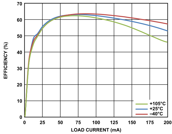
Figure 19. Typical Efficiency at 3.3 V In to 5 V Out over Temperature with 1:3 Coilcraft Transformer (CR7984-CL) at 500 kHz f_{SW}
