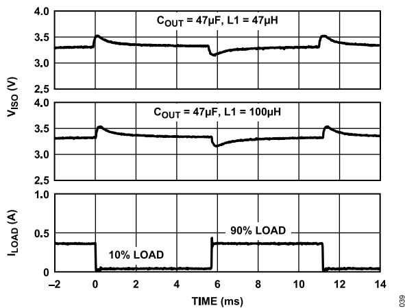
Figure 39. Typical V_{ISO} Load Transient Response 5 V Input to 3.3 V Output at 10% to 90% of 400 mA Load at 500 kHz f_{SW} with 0.1 \mu F Feedback Capacitor
