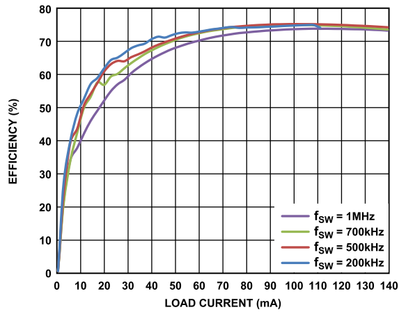
Figure 20. 5 V Input to 15 V Output Efficiency at Various Switching Frequencies with 1:3 Coilcraft Transformer (CR7984-CL)
