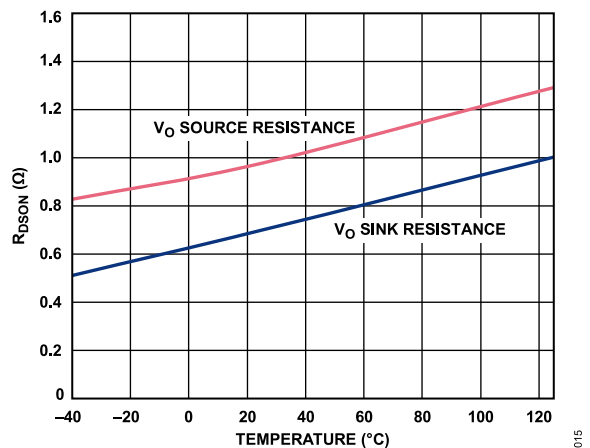
Figure 15. Typical Output Resistance ( R_{DS(on)} ) vs. Temperature, V_{DD2} = 12\text{ V}
