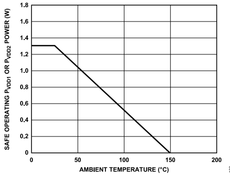
Figure 2. ADuM3123 Thermal Derating Curve, Dependence of Safety-Limiting Values on Case Temperature, per DIN EN IEC 60747-17 (VDE 0884-17)
