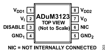
Figure 3. Pin Configuration
