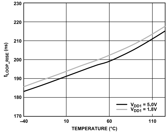
Figure 18. t_{LOOP\_RISE} vs. Temperature ( R_{SLOPE} = 47 k\Omega )
