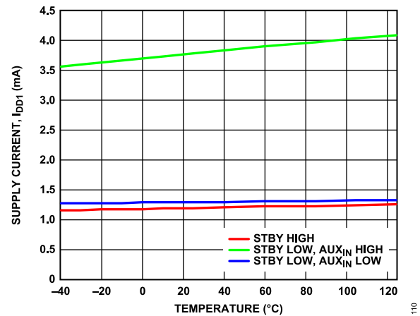
Figure 10. Supply Current, I_{DD1} vs. Temperature (Inputs Idle, V_{DD1} = 5\text{ V} )
