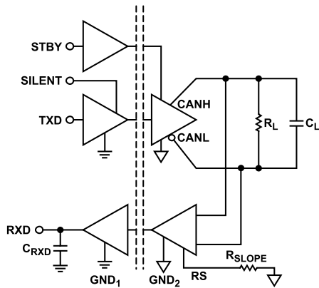
Figure 22. Receiver Voltage Measurement
