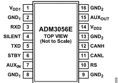
Figure 7. Pin Configuration
