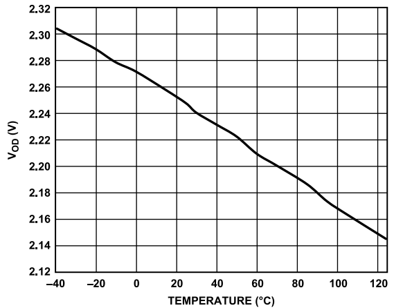
Figure 19. V_{OD} vs. Temperature
