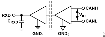
Figure 22. Receiver Voltage Measurement
