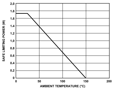
Figure 6. Thermal Derating Curve, Dependence of Safety Limiting Power Values with Ambient Temperature per DIN EN IEC 60747-17 (VDE 0884-17)
