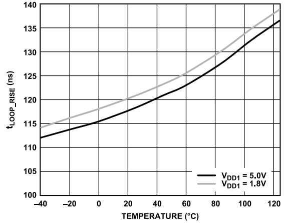
Figure 17. t_{LOOP\_RISE} vs. Temperature ( R_{SLOPE} = 0 \Omega )
