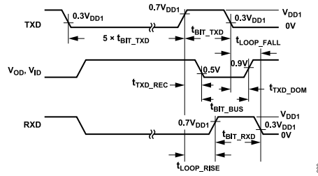
Figure 2. Driver/Receiver Timing Diagram
