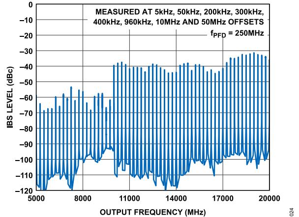
Figure 24. Worst Case Integer Boundary Spurs (IBS) Level vs. Output Frequency with f_{PFD} = 250 MHz
