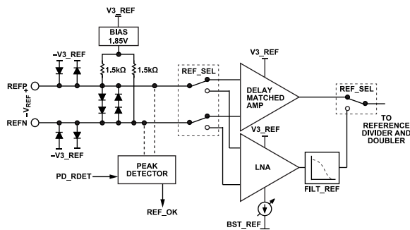
Figure 46. Reference Input Stage
