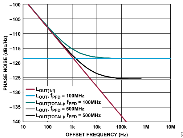
Figure 73. Theoretical In-Band Phase Noise, f_{OUT} = 10 GHz
