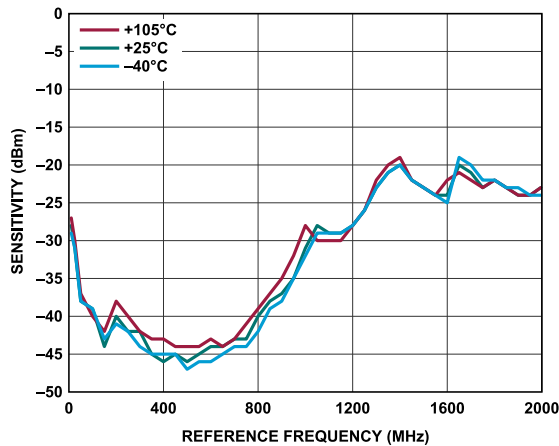
Figure 33. Reference Doubler Sensitivity for LNA Buffer at Various Temperatures
