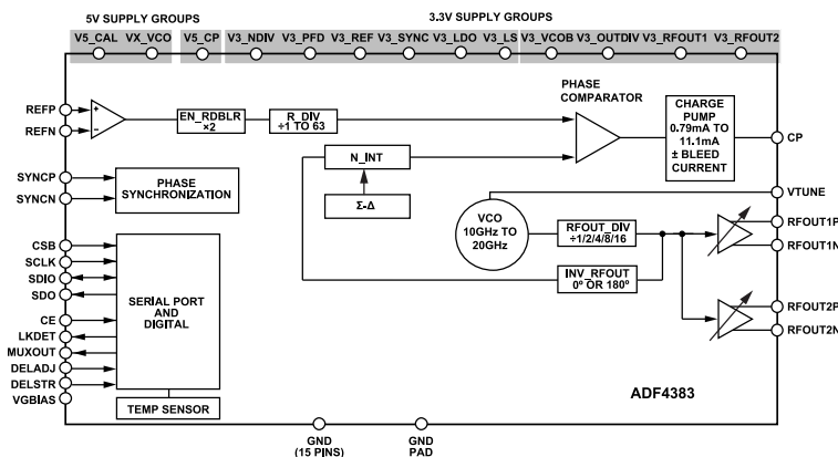
Figure 1. ADF4383 Functional Block Diagram
