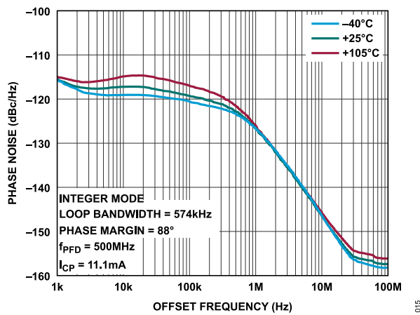
Figure 15. Closed-Loop Phase Noise vs. Offset Frequency at RFOUT = 14 GHz Across Temperatures
