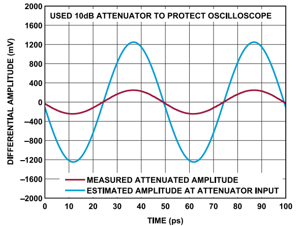
Figure 41. Differential Amplitude vs. Time at RFOUT = 20 GHz
