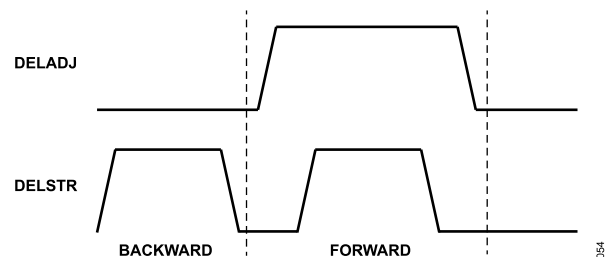
Figure 59. DELSTR and DELADJ Timing Diagrams
