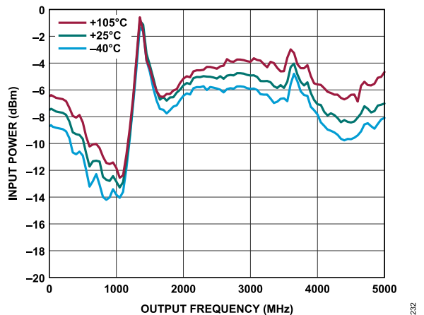
Figure 29. Minimum Input Signal for REF_OK = 1 for LNA Buffer at Various Temperatures
