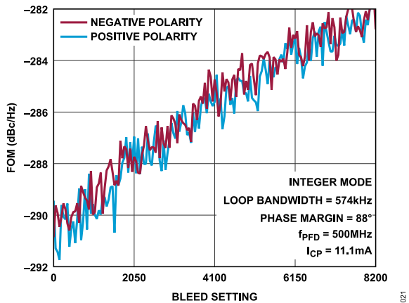
Figure 21. FOM, L_{1/f} Integer Mode vs. Bleed Setting, f_{PFD} = 500 MHz, R_{FOUT} = 20 GHz
