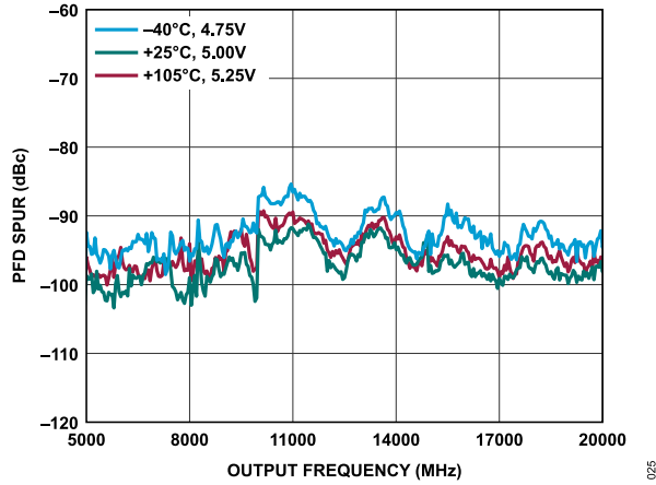
Figure 25. PFD Spur vs. Output Frequency at Various Temperatures and Voltages
