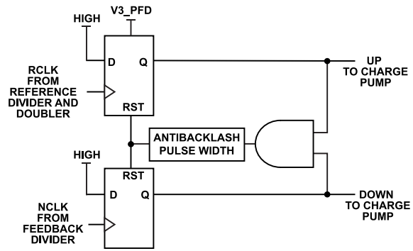
Figure 47. Simplified PFD Schematic
