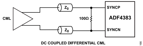
Figure 69. DC-Coupled Differential CML (Set SYNC_SEL = 0)
