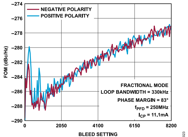
Figure 23. FOM, L_{1/f} Fractional Mode vs. Bleed Setting, f_{PFD} = 250 MHz, R_{FOUT} = 19.9 GHz
