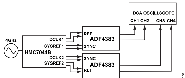
Figure 75. Timed Synchronization Configuration
