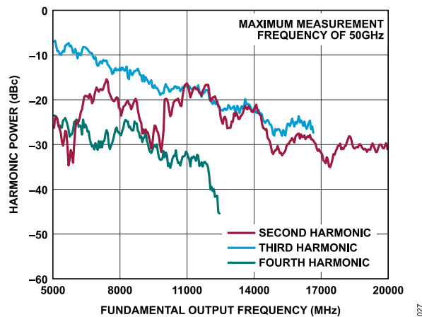
Figure 27. Harmonic Power vs. Fundamental Output Frequency
