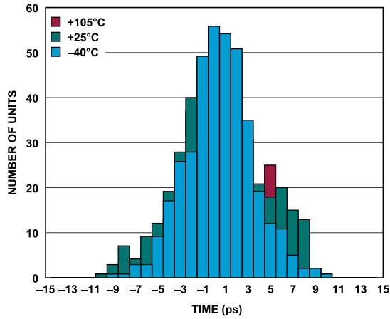
Figure 37. Normalized Propagation Delay ( t_{PD} ) Histogram
