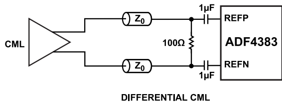
Figure 68. Differential CML
