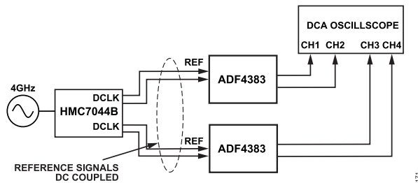
Figure 74. EZSync Configuration
