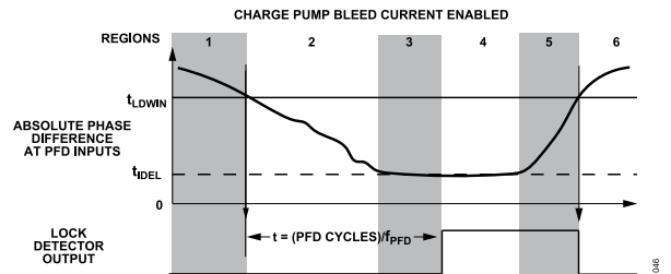
Figure 51. Lock Detector Timing, Bleed Current Enabled
