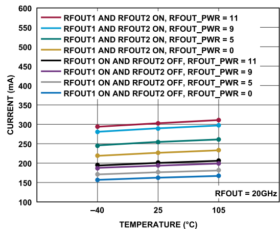
Figure 42. 3.3 V Supply Group 2 Current at Various Output Settings Across Temperature
