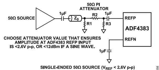
Figure 64. Single-Ended 50 \Omega Source ( V_{\text{REF}} < 2.6 \text{ V p-p} )
