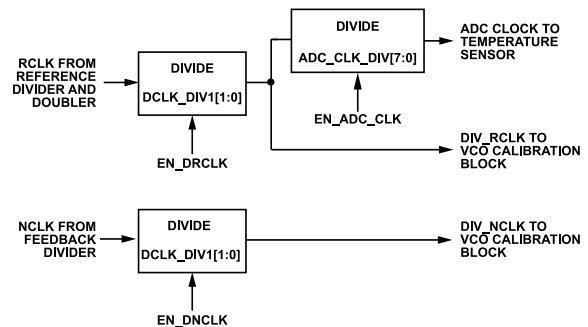
Figure 57. VCO Calibration Dividers
