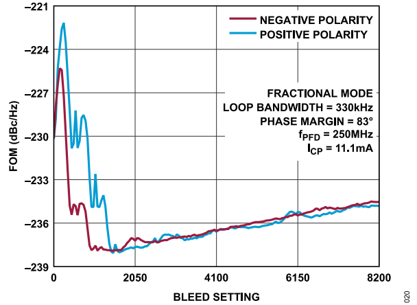
Figure 22. FOM, L_{NORM} Fractional Mode vs. Bleed Setting, f_{PFD} = 250 MHz, R_{FOUT} = 19.9 GHz
