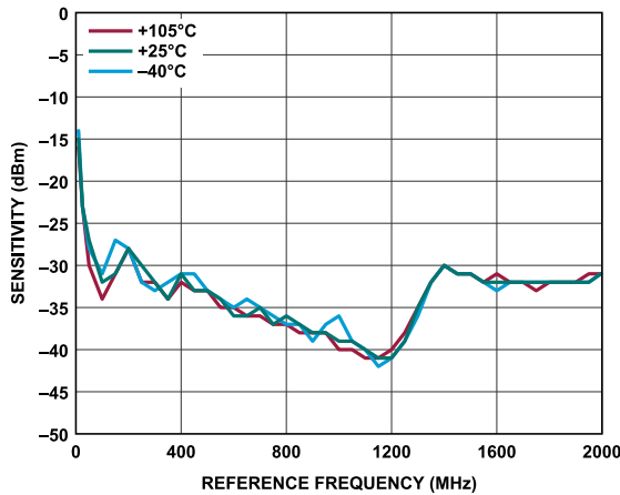
Figure 32. Reference Doubler Sensitivity for DMA Buffer at Various Temperatures
