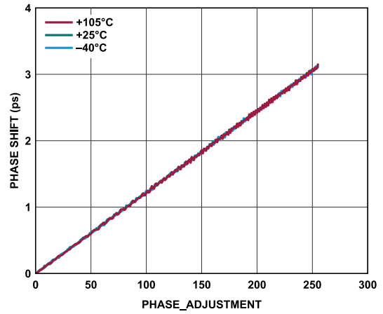
Figure 40. Phase Shift vs. PHASE_ADJUSTMENT for Various Temperatures
