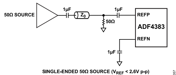
Figure 63. Single-Ended 50 \Omega Source ( V_{\text{REF}} < 2.6 \text{ V p-p} )
