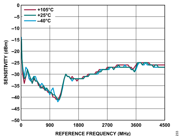
Figure 30. Reference Sensitivity for DMA Buffer at Various Temperatures
