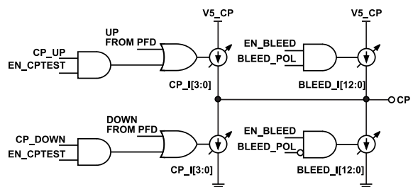
Figure 48. Simplified Charge Pump Schematic
