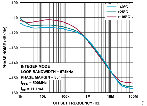
Figure 16. Closed-Loop Phase Noise vs. Offset Frequency at RFOUT = 20 GHz VCO Frequency Across Temperatures
