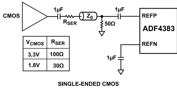
Figure 65. Single-Ended CMOS (R SER Is the Series Resistance.)
