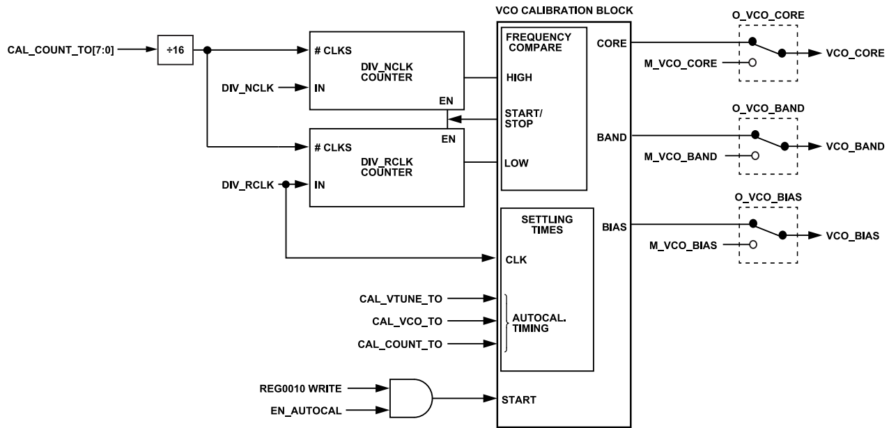
Figure 58. VCO Calibration Block
