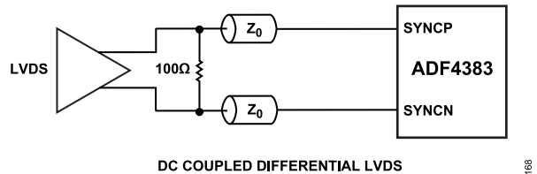
Figure 71. DC-Coupled Differential LVDS (Set SYNC_SEL = 1)
