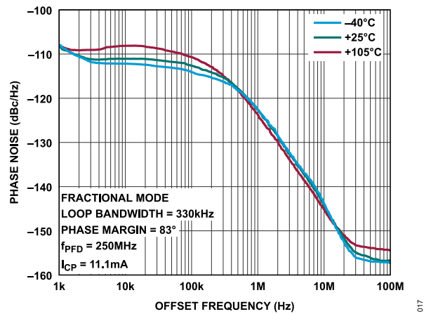
Figure 17. Closed-Loop Phase Noise vs. Offset Frequency at 19.9 GHz VCO Frequency Across Temperatures
