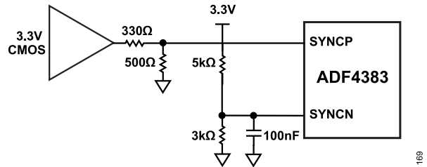
Figure 72. DC-Coupled 3.3 V Single-Ended Logic to LVDS Input (Set SYNC_SEL = 1)
