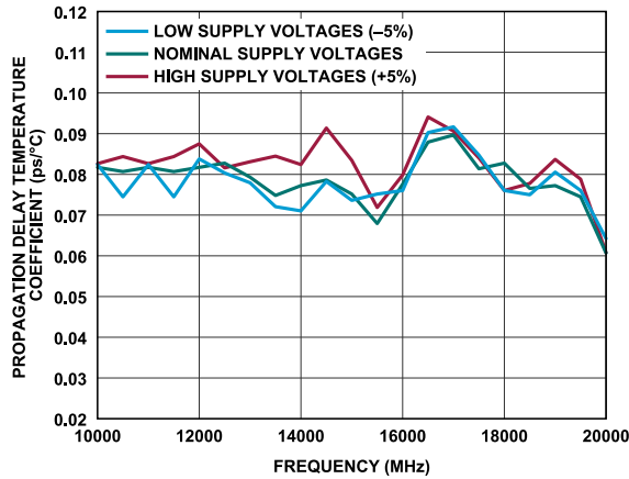
Figure 38. Propagation Delay Temperature Coefficient vs. Frequency
