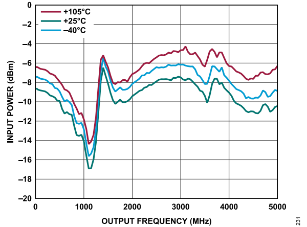
Figure 28. Minimum Input Signal for REF_OK = 1 for Delayed Match Amplifier (DMA) Buffer at Various Temperatures
