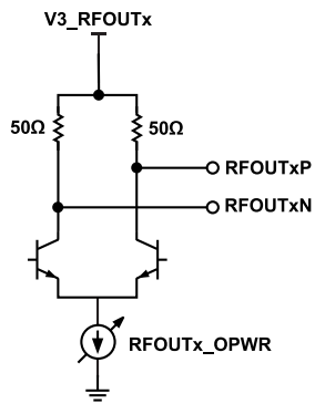
Figure 60. Simplified RF Output Buffer Schematic
