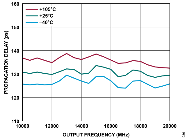
Figure 36. Propagation Delay vs. Output Frequency at Various Temperatures
