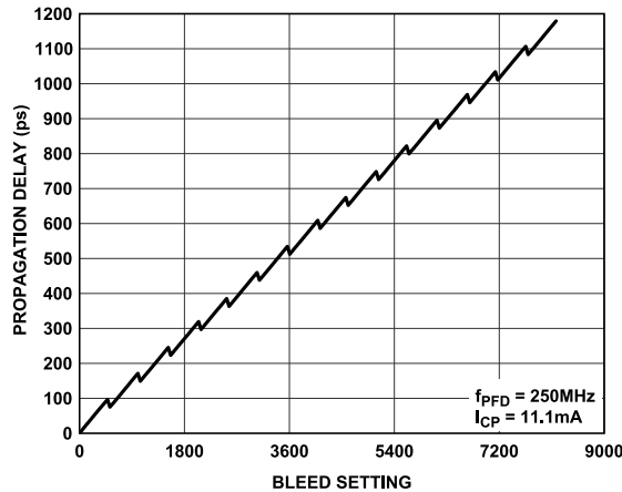
Figure 39. Propagation Delay vs. Bleed Setting
