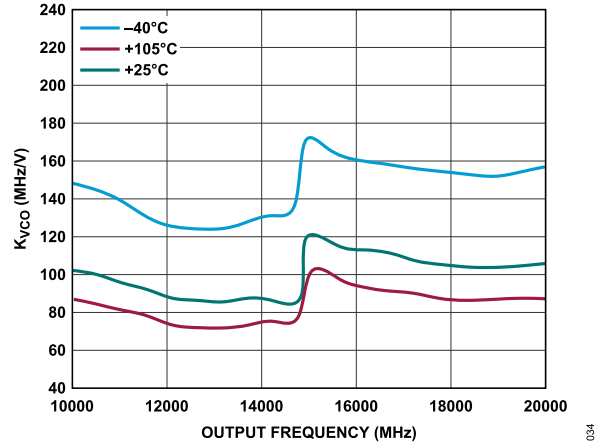
Figure 34. K_{VCO} vs. Output Frequency at Various Temperatures
