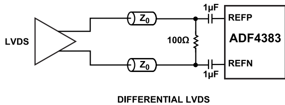
Figure 67. Differential LVDS
