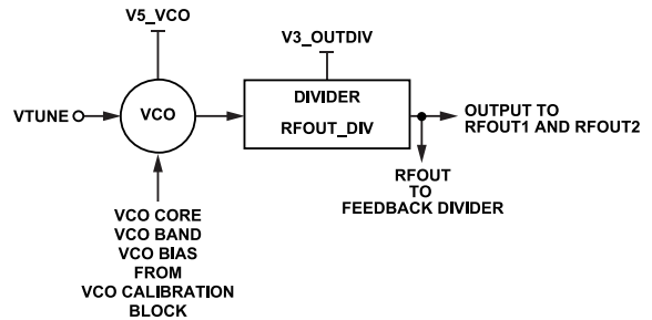
Figure 56. VCO and Clock Output Divider
