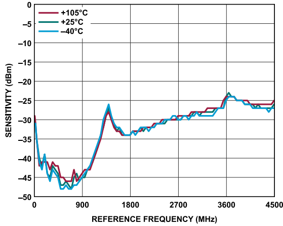
Figure 31. Reference Sensitivity for LNA Buffer at Various Temperatures
