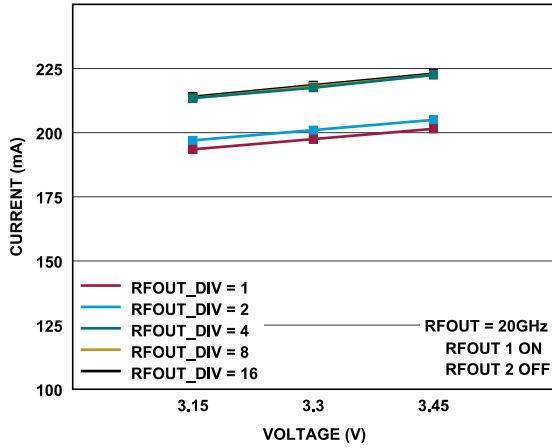
Figure 43. 3.3 V Supply Group 2 Current at Various Power Supply Voltages and RFOUT_DIV Settings
