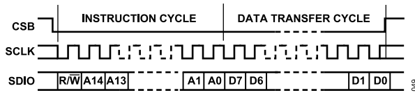
Figure 54. Serial Interface, MSB First (LSB_FIRST = 0)
