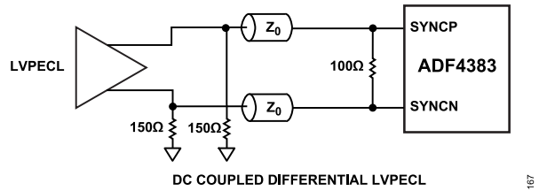
Figure 70. DC-Coupled Differential LVPECL (Set SYNC_SEL = 0)
