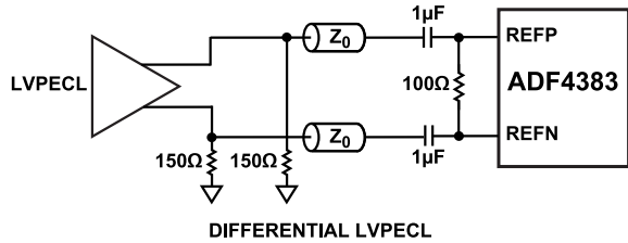
Figure 66. Differential, Low Voltage, Positive Emitter-Coupled Logic (LVPECL)
