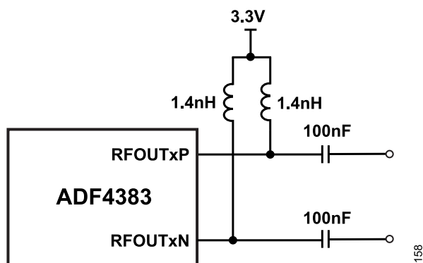
Figure 61. RFOUT Interface Schematic
