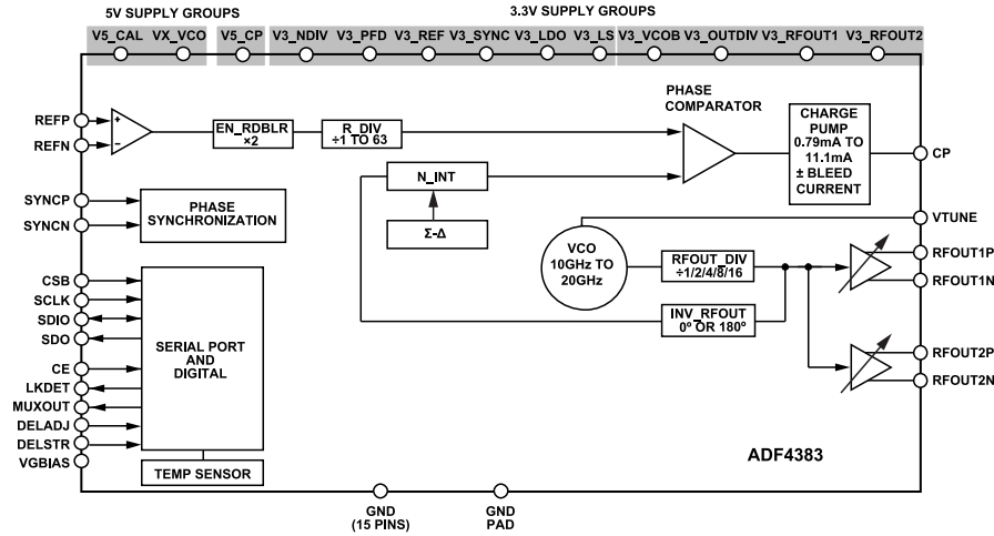
Figure 45. PLL Loop Diagram
