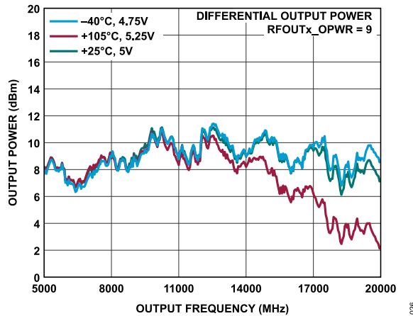
Figure 26. Differential Output Power vs. Output Frequency at Various Temperatures and Voltages
