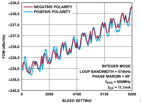
Figure 20. FOM, L_{NORM} Integer Mode vs. Bleed Setting, f_{PFD} = 500 MHz, R_{FOUT} = 20 GHz
