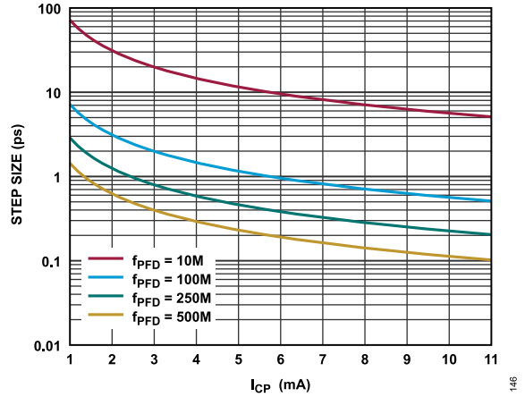
Figure 49. Bleed Current Delay Step Size
