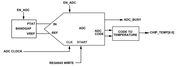
Figure 53. Temperature Sensor
