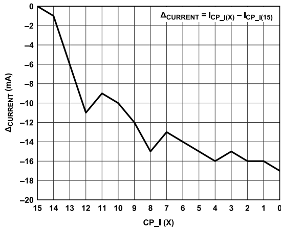
Figure 44. 5 V Delta Supply Current ( \Delta_{CURRENT} ) at Various CP_I Settings
