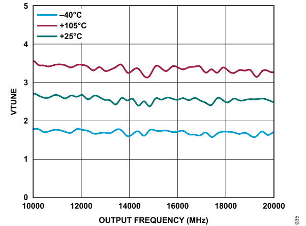
Figure 35. V_{TUNE} vs. Output Frequency at Various Temperatures
