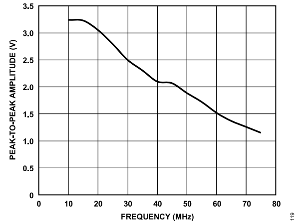
Figure 19. Amplitude vs. Toggle Rate with 10 pF Load, 3.3 V (Weak Mode) CMOS
