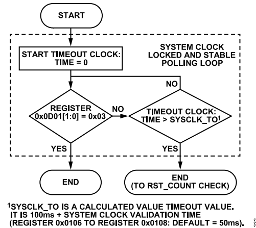
Figure 36. AD9558 System Clock Initialization Subprocess Flowchart
