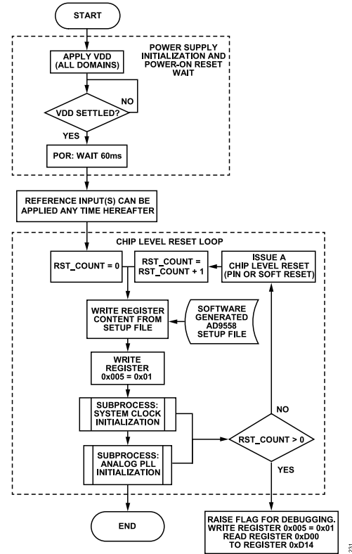
Figure 35. AD9558 Initialization Flowchart
