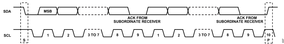
Figure 57. Acknowledge Bit
