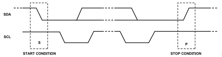
Figure 56. Start and Stop Conditions
