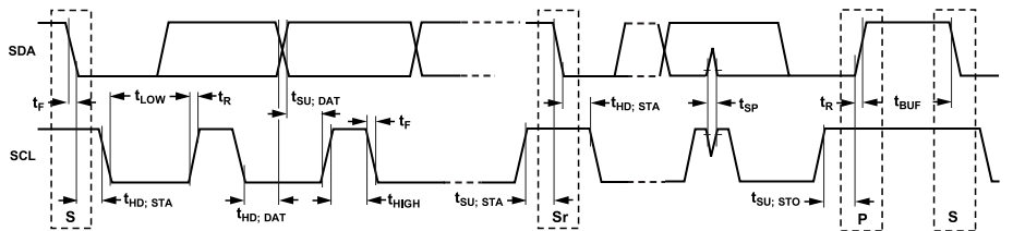
Figure 60. I 2 C Serial Port Timing
