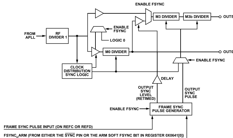
Figure 45. Frame Synchronization in One-Shot Mode
