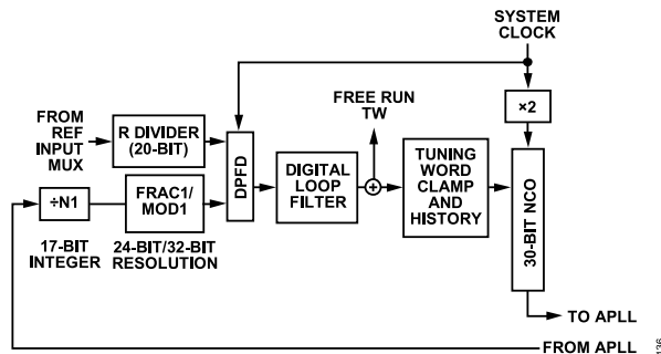
Figure 39. Digital PLL Core
