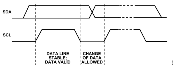
Figure 55. Valid Bit Transfer
