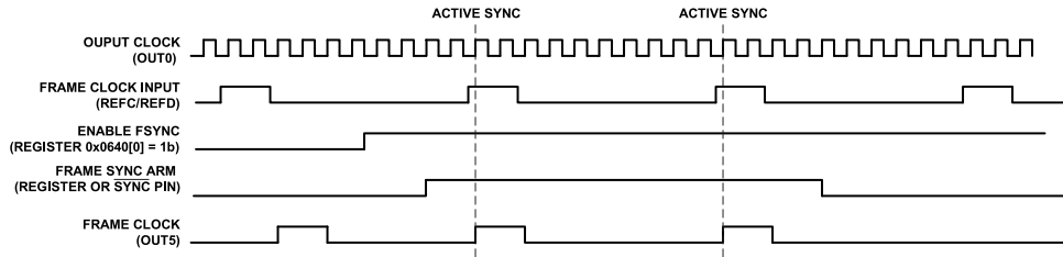
Figure 44. Frame Synchronization in Level Sensitive Mode
