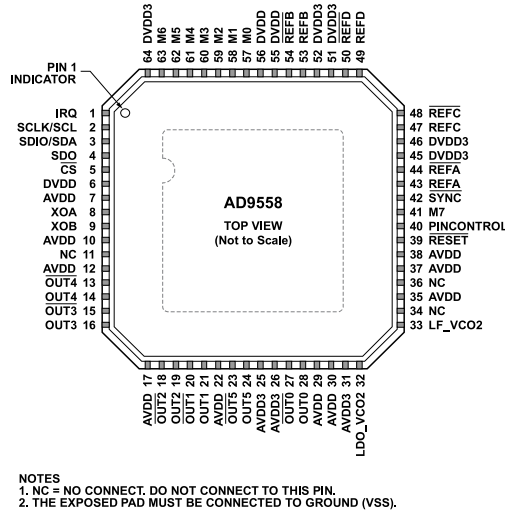
Figure 2. Pin Configuration
