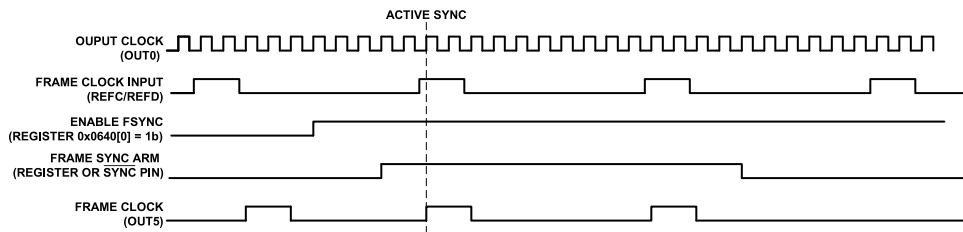
Figure 44. Frame Synchronization in Level Sensitive Mode
