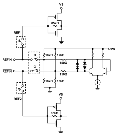
Figure 44. REF1N Equivalent Circuit for Non-XTAL Mode
