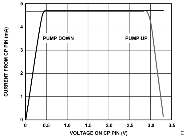
Figure 9. Charge Pump Characteristics at VCP = 3.3 V
