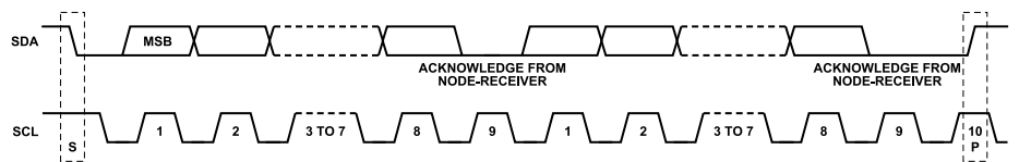
Figure 59. Acknowledge Bit
