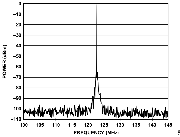
Figure 13. PFD/CP Spurs; 122.88 MHz; PFD = 15.36 MHz; LBW = 127 kHz; I_{CP} = 3.0 mA; f_{VCO} = 2580 MHz
