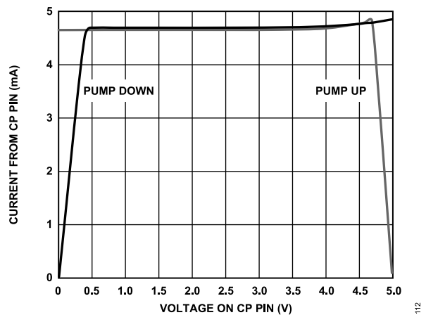
Figure 10. Charge Pump Characteristics at VCP = 5.0 V
