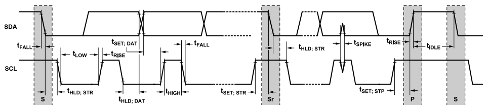
Figure 62. I 2 C Serial Port Timing
