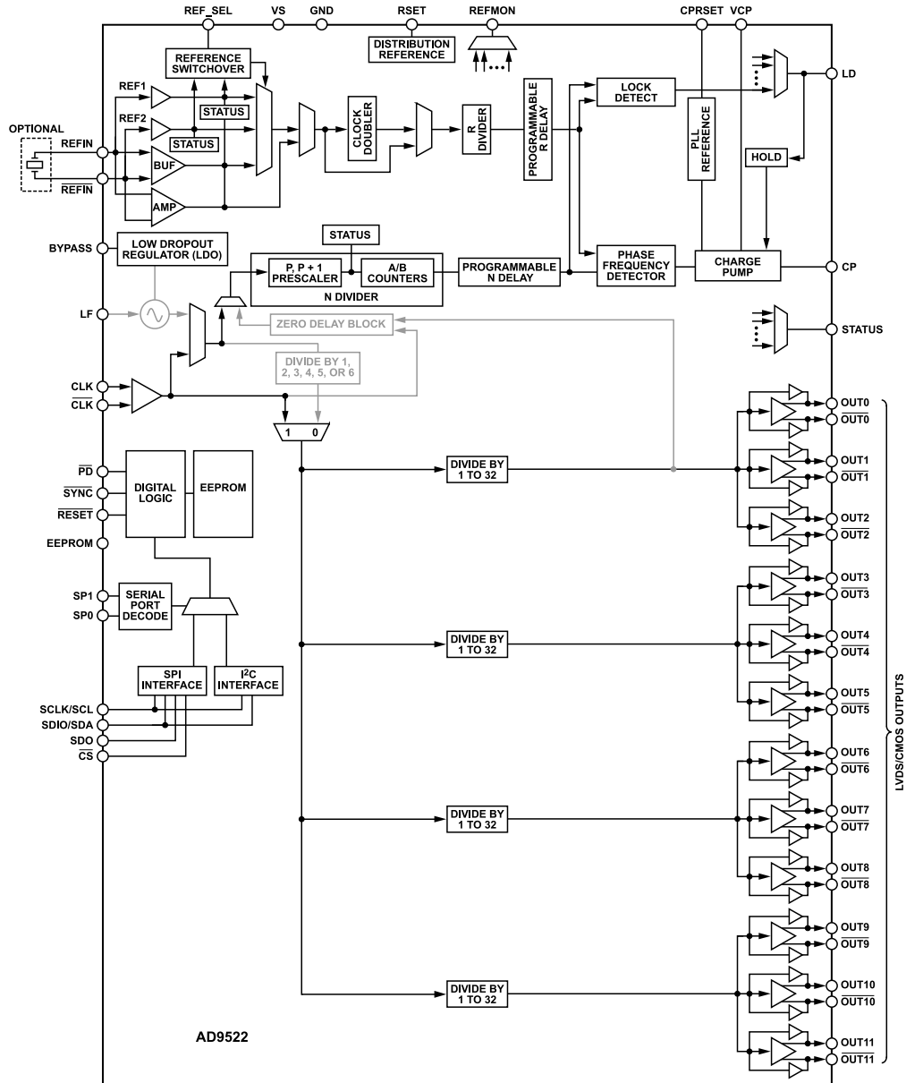
Figure 37. Clock Distribution or External VCO < 1600 MHz (Mode 1)
