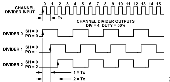
Figure 52. Effect of Coarse Phase Offset (or Delay)
