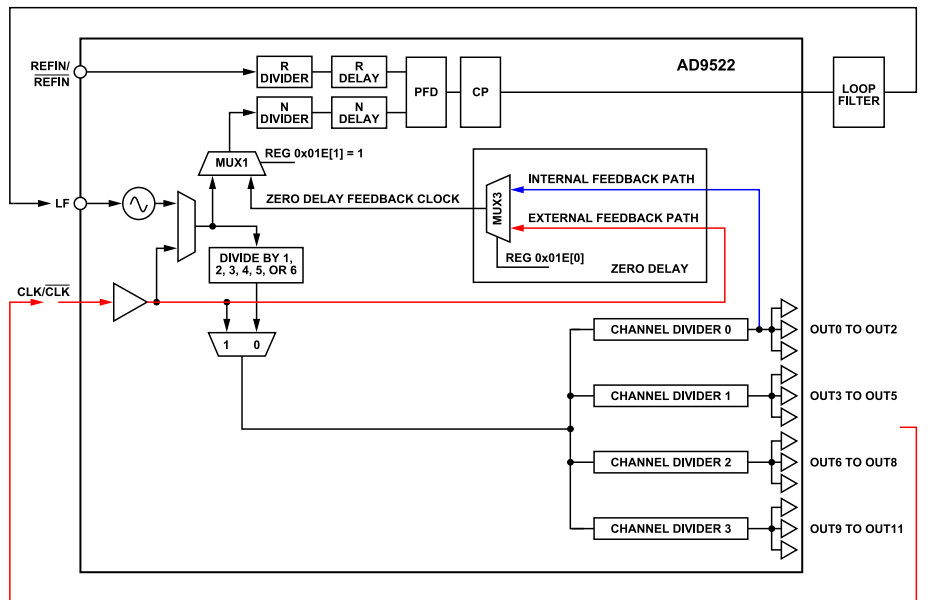
Figure 50. Zero Delay Function
