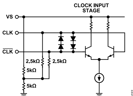
Figure 47. CLK Equivalent Input Circuit
