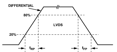
Figure 3. LVDS Timing, Differential
