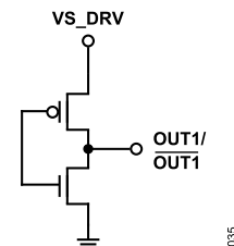
Figure 56. CMOS Equivalent Output Circuit
