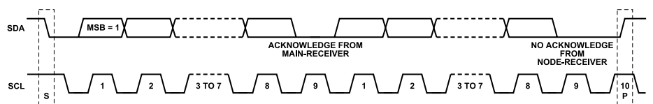
Figure 61. Data Transfer Process (Main Read Mode, 2-Byte Transfer Used for Illustration)
