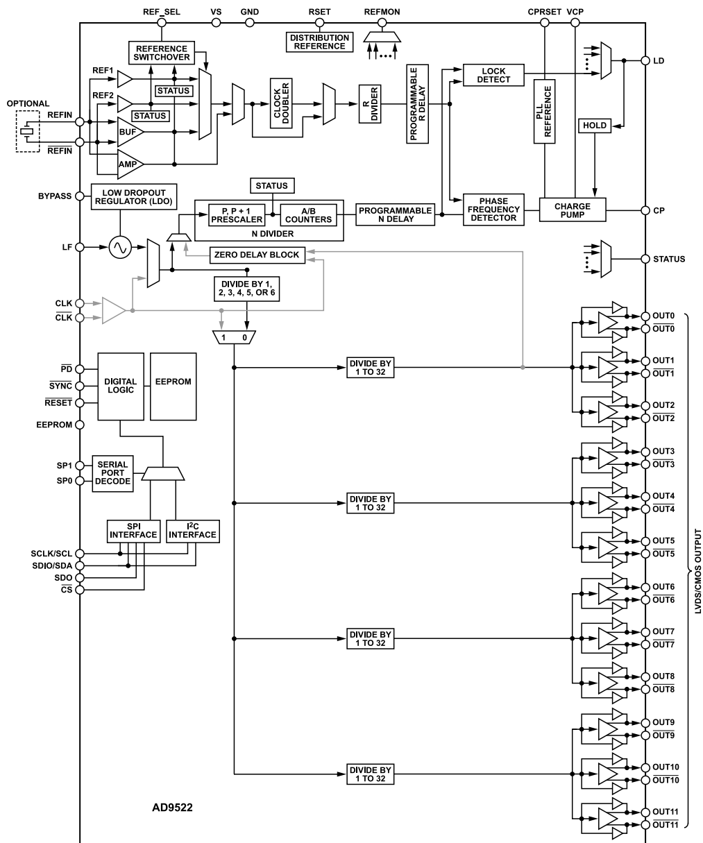
Figure 36. Internal VCO and Clock Distribution (Mode 0)
