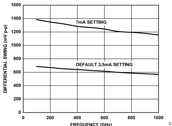
Figure 20. LVDS Differential Voltage Swing vs. Frequency Output Terminated 100 Ω Across Differential Pair
