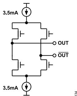
Figure 55. LVDS Output Simplified Equivalent Circuit with 3.5 mA Typical Current Source
