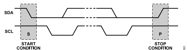
Figure 58. Start and Stop Conditions
