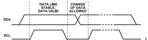
Figure 57. Valid Bit Transfer
