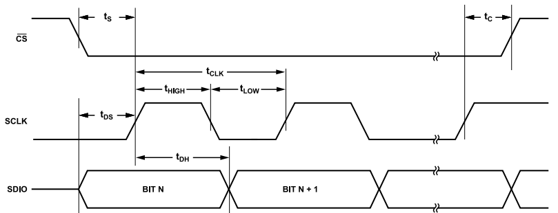
Figure 70. Serial Control Port Timing—Write
