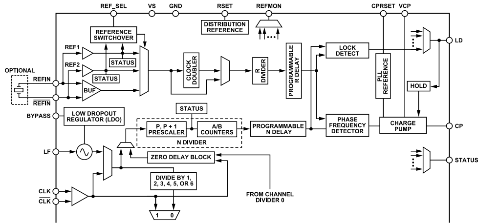
Figure 39. PLL Functional Block Diagram
