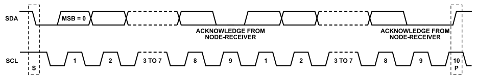
Figure 60. Data Transfer Process (Main Write Mode, 2-Byte Transfer Used for Illustration)
