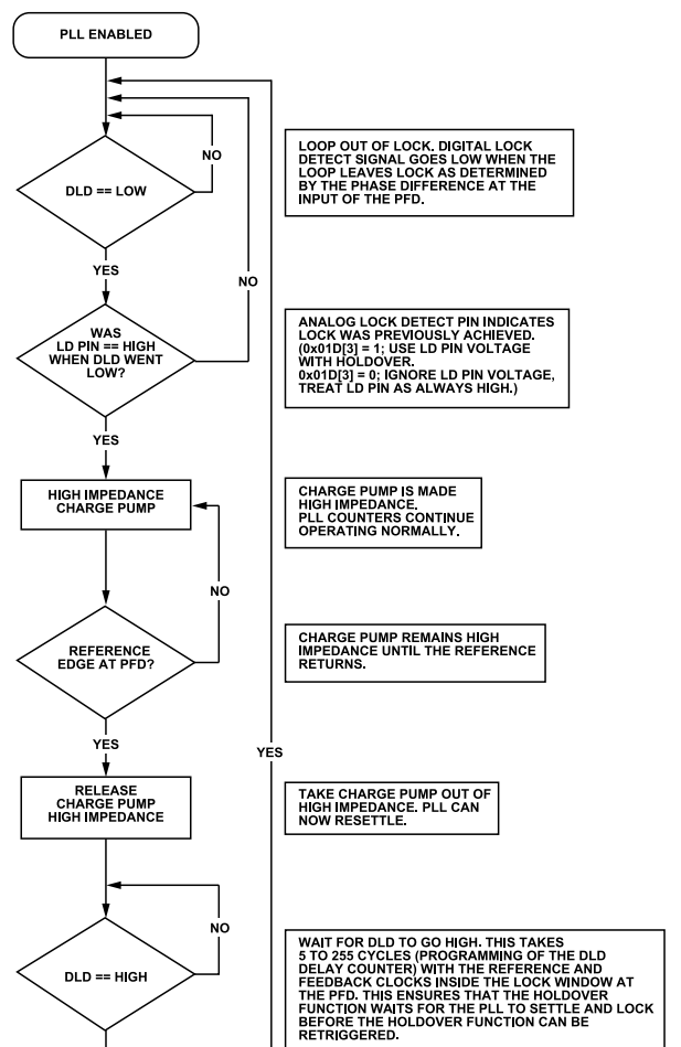
Figure 48. Flowchart of Automatic/Internal Holdover Mode
