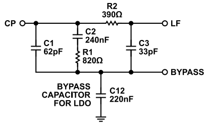
Figure 33. PLL Loop Filter Used for Clock Generation Plot (See Figure 30 )
