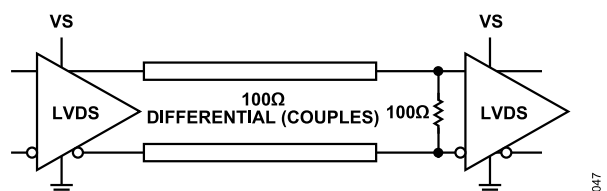
Figure 72. LVDS Output Termination
