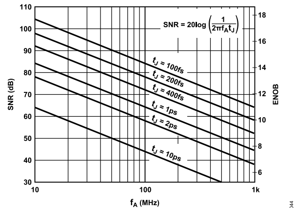
Figure 71. SNR and ENOB vs. Analog Input Frequency
