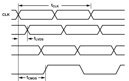
Figure 2. CLK/CLK to Clock Output Timing, DIV = 1
