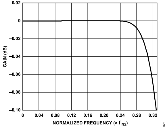
Figure 55. Pass-Band Detail of HB2
