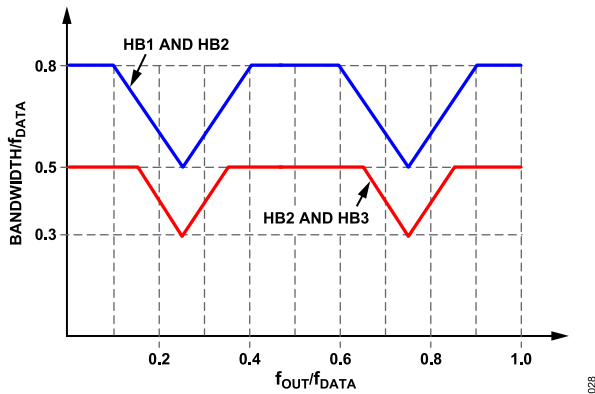
Figure 58. Signal Bandwidth vs. Center Frequency of the Output Signal, 4x Interpolation
