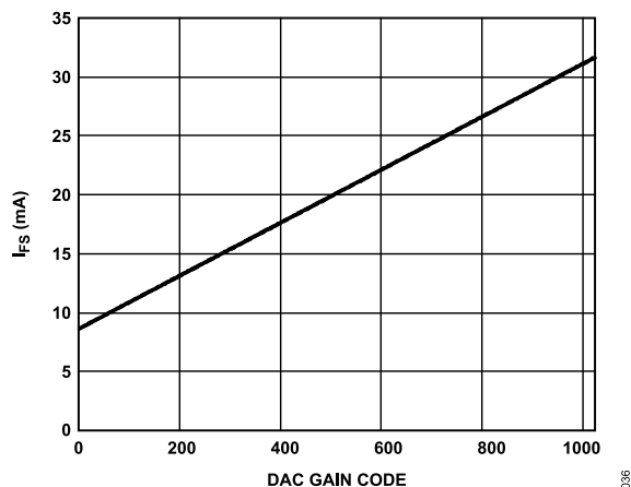
Figure 67. DAC Full-Scale Current vs. DAC Gain Code
