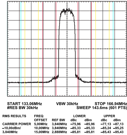
Figure 34. Four-Carrier W-CDMA ACLR Performance, IF ≈150 MHz
