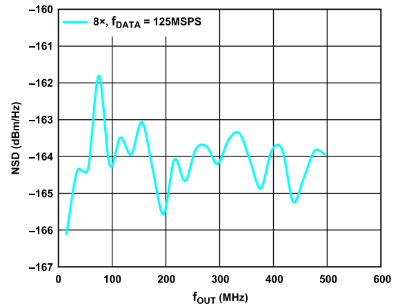
Figure 27. Eight-Tone NSD vs. f_{OUT} over Interpolation Rate and f_{DATA} , Digital Scale = 0 dBFS, f_{SC} = 20 mA, PLL On
