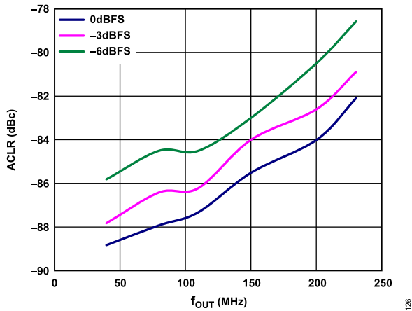
Figure 29. One-Carrier W-CDMA ACLR vs. f_{OUT} over f_{DAC} , Alternate Channel, PLL Off
