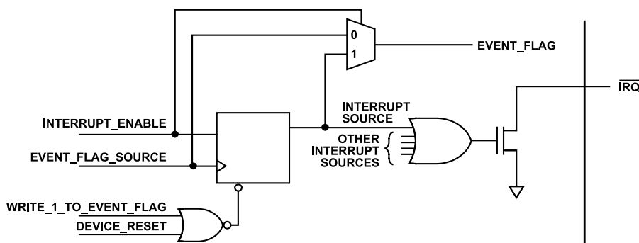
Figure 86. Simplified Schematic of \overline{\text{IRQ}} Circuitry
