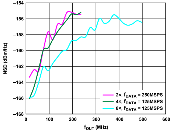
Figure 22. One-Tone NSD vs. f_{OUT} over Interpolation Rate and f_{DATA} , Digital Scale = 0 dBFS, f_{SC} = 20 mA, PLL Off
