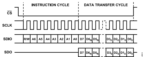
Figure 38. Serial Register Interface Timing, MSB First
