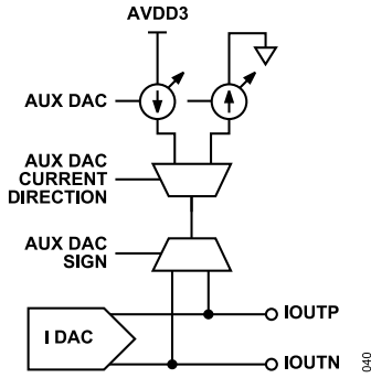
Figure 72. Auxiliary DAC Structure
