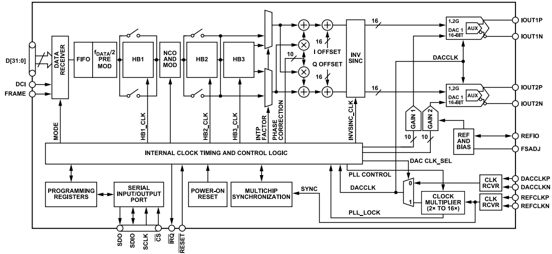
Figure 2. AD9125 Functional Block Diagram
