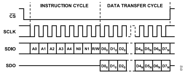
Figure 39. Serial Register Interface Timing, LSB First
