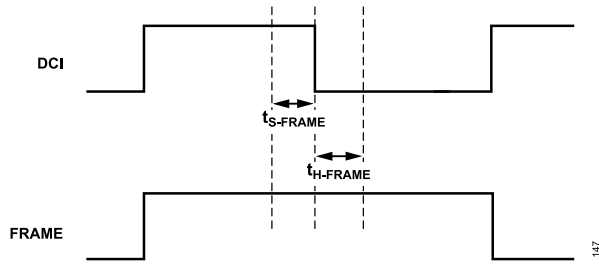
Figure 46. Timing Diagram for Frame input
