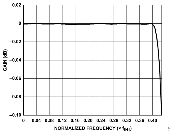
Figure 52. Pass-Band Detail of HB1
