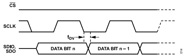
Figure 41. Timing Diagram for Serial Port Register Read
