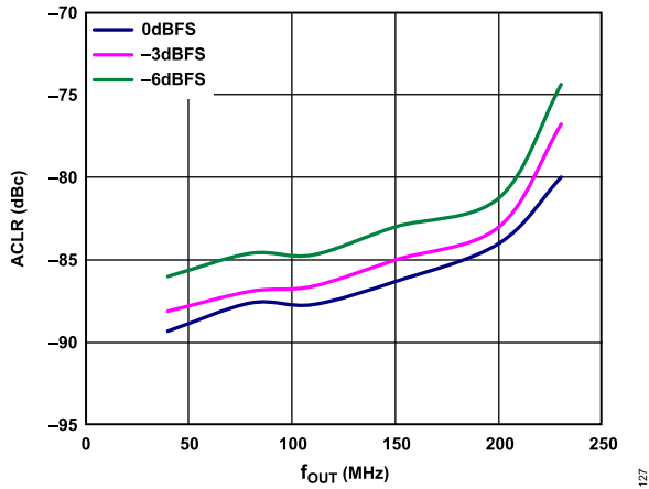
Figure 30. One-Carrier W-CDMA ACLR vs. f_{OUT} over f_{DAC} , Second Alternate Channel, PLL Off
