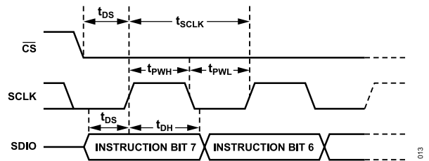
Figure 40. Timing Diagram for Serial Port Register Write ( t_{DS} to t_{D}\overline{CS} )
