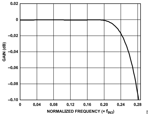
Figure 56. Pass-Band Detail of HB3
