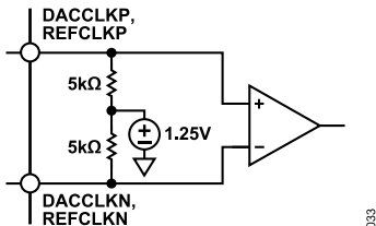
Figure 63. Clock Receiver Input Equivalent Circuit
