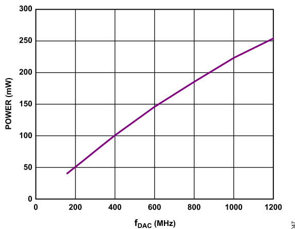
Figure 79. DVDD18 Power Dissipation vs. f_{\text{DAC}} Due to Inverse Sinc Filter
