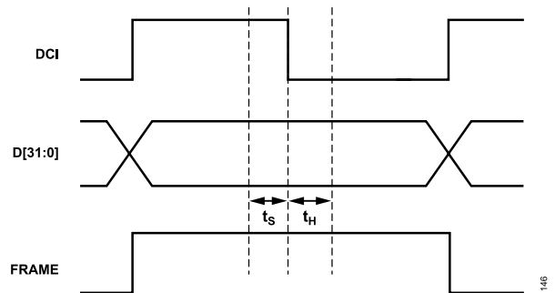
Figure 45. Timing Diagram for Input Data Ports
