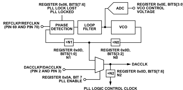
Figure 64. PLL Clock Multiplication Circuit
