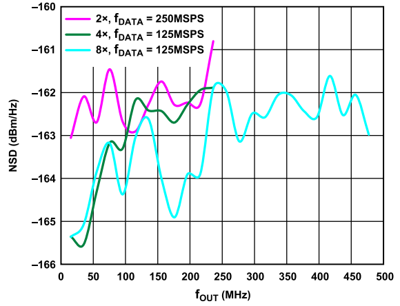
Figure 25. Eight-Tone NSD vs. f_{OUT} over Interpolation Rate and f_{DATA} , Digital Scale = 0 dBFS, f_{SC} = 20 mA, PLL Off
