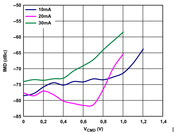
Figure 71. IMD vs. Common-Mode Output Voltage ( f_{OUT} = 161 \text{ MHz} , R_{LOAD} = 50 \Omega differential, I_{FS} = 10 \text{ mA} , 20 \text{ mA} , and 30 \text{ mA} )
