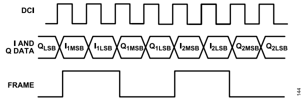
Figure 44. Timing Diagram for Byte Mode
