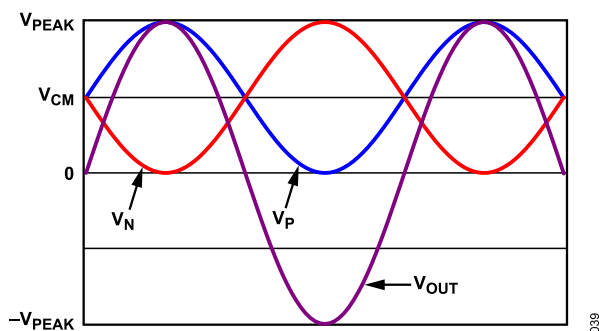
Figure 69. Voltage Output Waveforms
