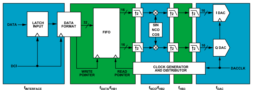
Figure 36. Defining Data Rates
