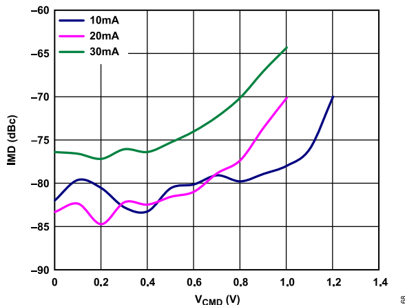
Figure 70. IMD vs. Common-Mode Output Voltage ( f_{OUT} = 61 \text{ MHz} , R_{LOAD} = 50 \Omega differential, I_{FS} = 10 \text{ mA} , 20 \text{ mA} , and 30 \text{ mA} )
