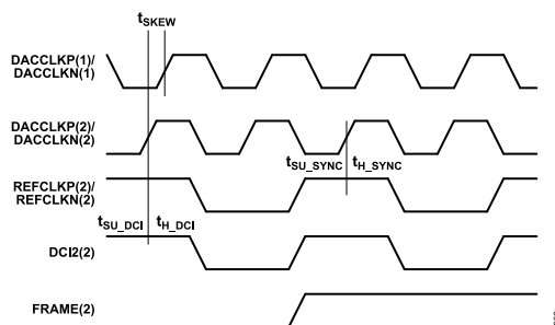
Figure 84. Data Rate Synchronization Signal Timing Requirements, 2× Interpolation
