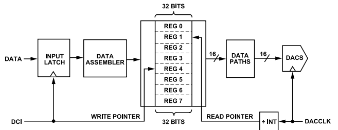
Figure 47. Block Diagram of Datapath Through FIFO
