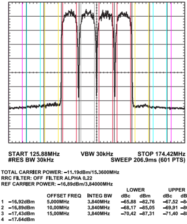
Figure 35. One-Carrier W-CDMA ACLR Performance, IF ≈150 MHz
