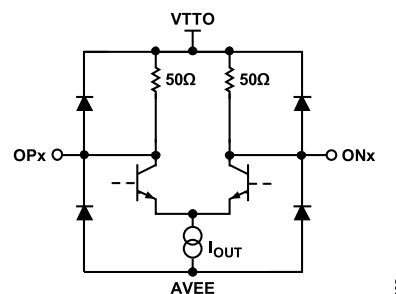
Figure 31. High Speed Output Simplified Schematic
