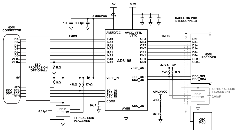
Figure 34. AD8195 Typical Application Simplified Schematic
