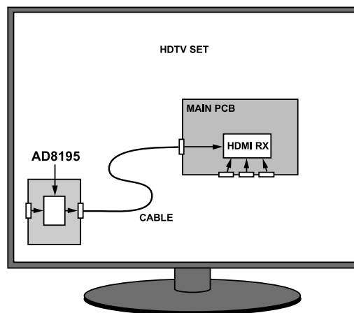
Figure 33. AD8195 as a Front Panel Buffer for an HDTV
