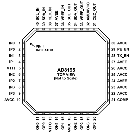
Figure 3. Pin Configuration
