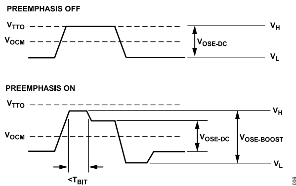
Figure 32. Preemphasis Pulse Response
