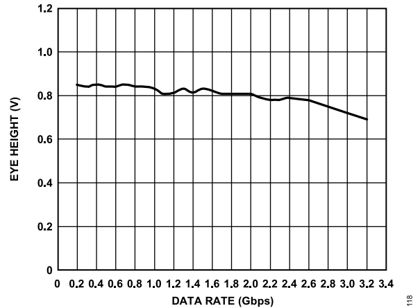
Figure 22. Eye Height vs. Data Rate
