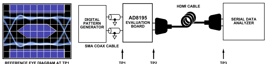
Figure 13. Test Circuit Diagram for Tx Eye Diagrams
