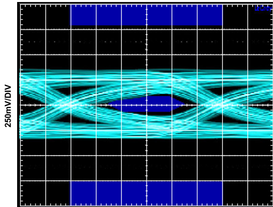
0.167UI/DIV AT 3.0Gbps
