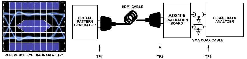
Figure 4. Test Circuit Diagram for Rx Eye Diagrams
