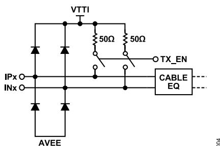
Figure 30. High Speed Input Simplified Schematic
