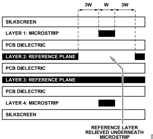
Figure 35. Example Board Stack-Up
