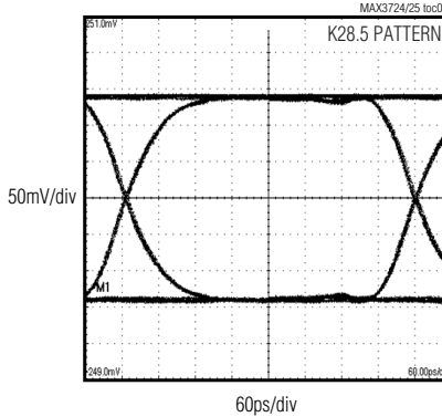
EYE DIAGRAM
