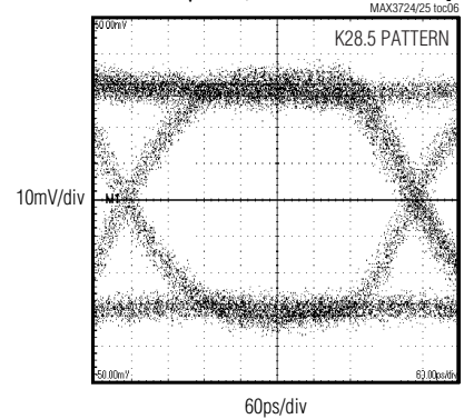
EYE DIAGRAM INPUT = 20μAp-p, DATA RATE = 2.1Gbps
