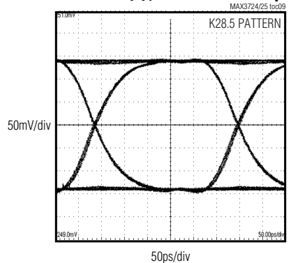
EYE DIAGRAM
