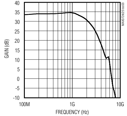
OPTICAL FREQUENCY RESPONSE (70μm InGaAs PHOTODIODE, INPUT -22dBm)
