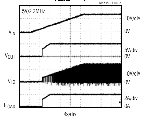
OUTPUT RESPONSE TO SLOW INPUT RAMP (LOAD = 2A) MAX16977 toc13
