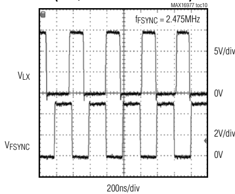
FSYNC TRANSITION FROM INTERNAL TO EXTERNAL FREQUENCY (3.3V/2.2MHz CONFIGURATION) MAX16977 toc10
