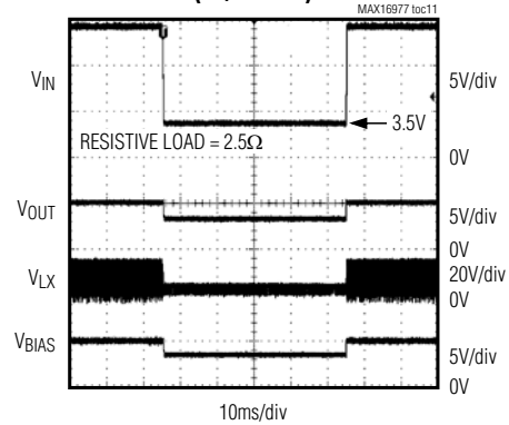
UNDERVOLTAGE PULSE (5V/2.2MHz) MAX16977 toc11
