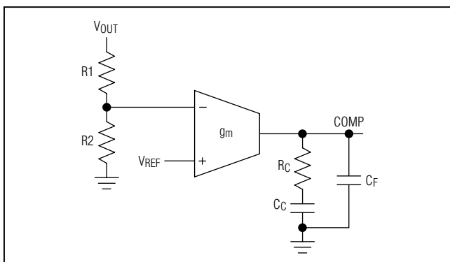
Figure 3. Compensation Network
