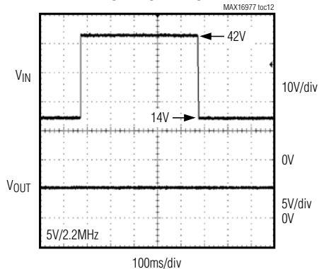
LOAD DUMP TEST MAX16977 toc12
