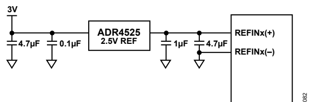
Figure 76. ADR4525 to ADFS7124-8 Connections
