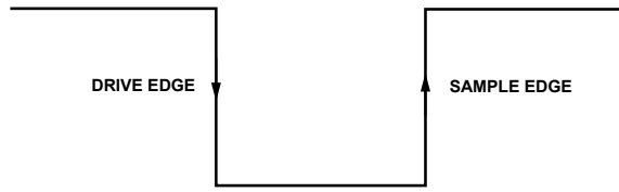
Figure 65. SPI Mode 3, SCLK Edges
