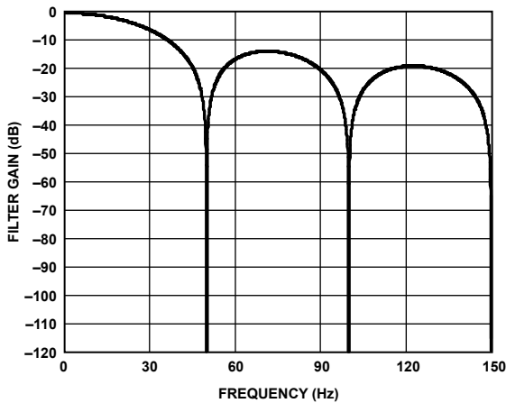
Figure 106. 50 Hz Rejection
