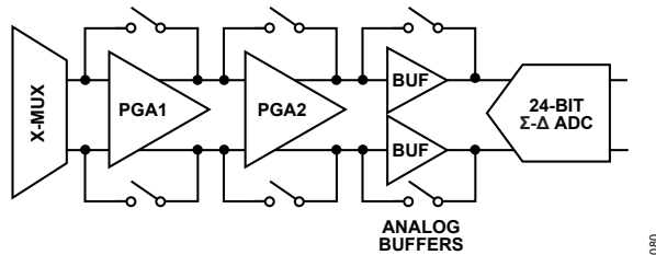
Figure 74. Programmable Gain Amplifier (PGA)
