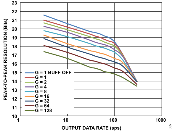
Figure 55. Peak-to-Peak Resolution vs. Output Data Rate, Sinc^3 + Sinc^1 Filter (Mid Power Mode)
