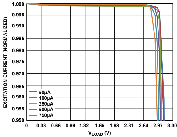
Figure 35. Output Compliance ( AV_{DD} = 3.3V )
