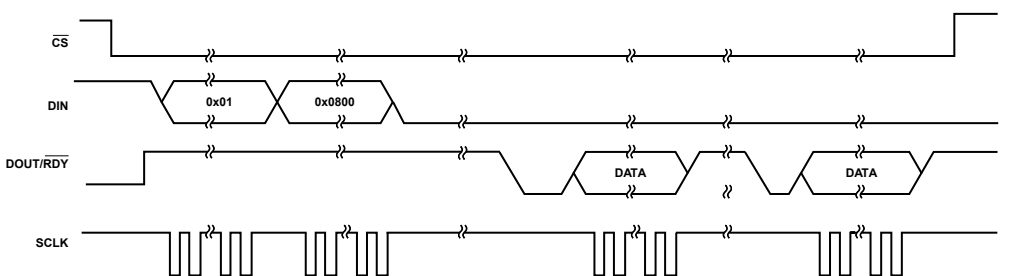
Figure 80. Continuous Read Configuration
