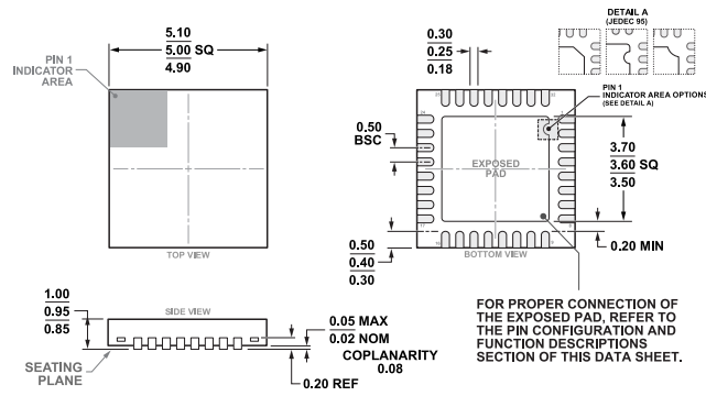
Figure 129. 32-Lead Lead Frame Chip Scale Package [LFCSP] 5 mm × 5 mm Body and 0.95 mm Package Height (CP-32-30) Dimensions shown in millimeters
