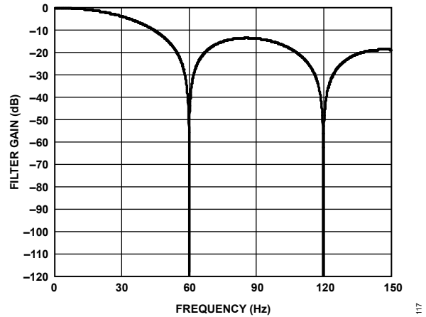
Figure 107. 60 Hz Rejection
